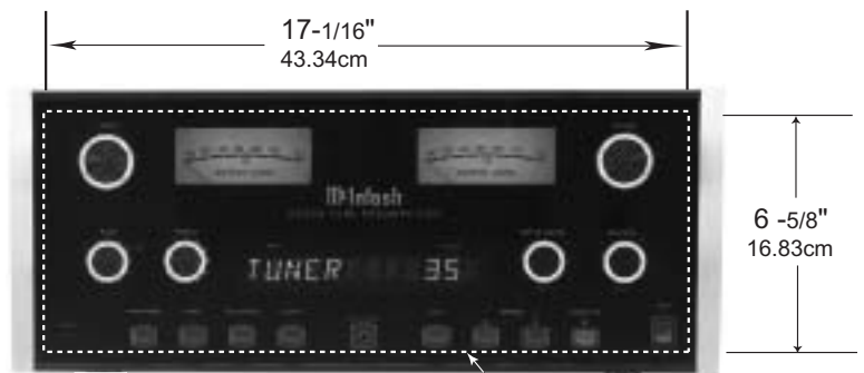
C2200 Front Panel Custom Cabinet Cutout
